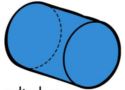
cylinder
