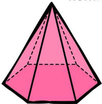
hexagonal pyramid
