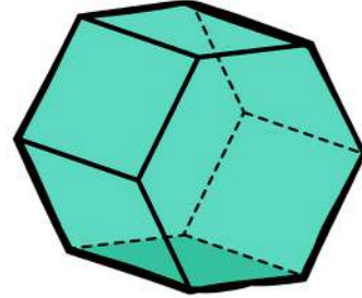
hexagonal prism
