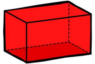
cuboid
