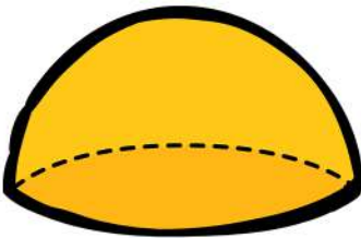
hemisphere
