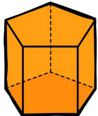
pentagonal prism
